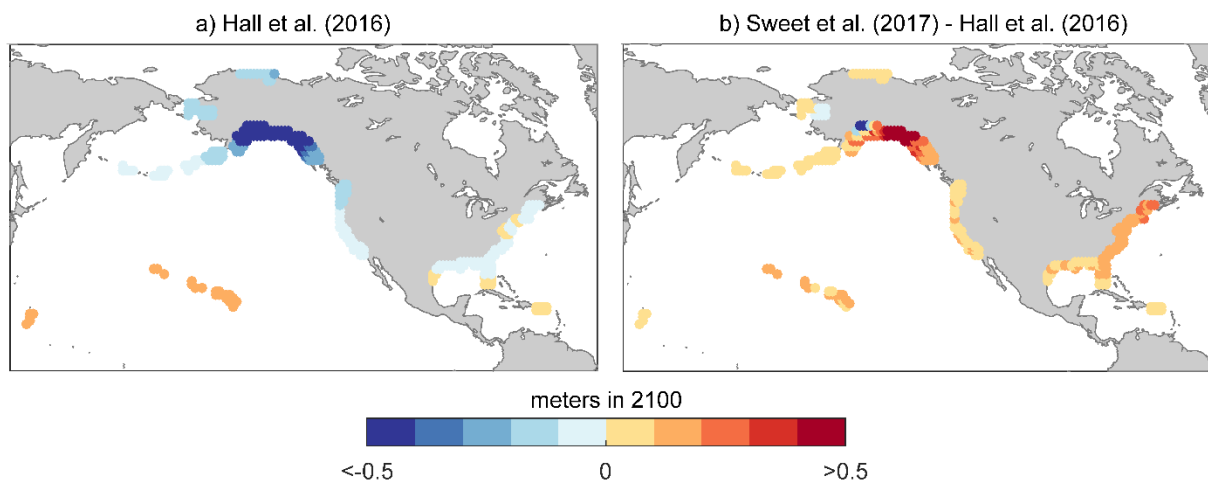
Figure 11. a) Median climate-related RSL amounts under the Intermediate (1-m GMSL rise) scenario in year 2100 of Hall et al. (2016) (with all grid values shown with GMSL amount [1.0 m] removed) and b) difference between RSL in this study's (Sweet et al., 2017) Intermediate scenario as shown in Figure 9 and Hall et al. (2016) results shown in a).
