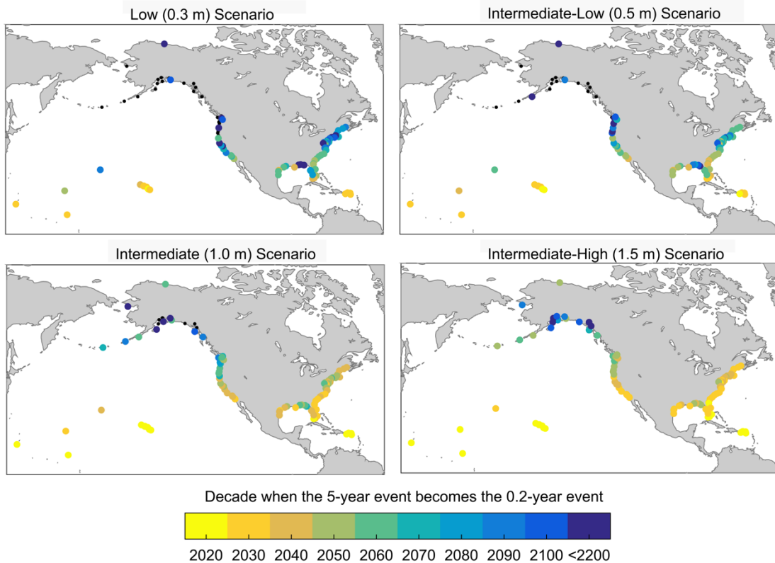
Figure 16. The decade ( \pm 5 years about the year shown in the legend) when the flood event with a 5-year recurrence interval (20% annual chance) becomes a 0.2-year recurrence interval (or annual probability increases 25-fold) under location-specific RSL associated with the a) Low b) Intermediate-Low, c) Intermediate and d) Intermediate-High scenarios. Black dots are locations where the 5-year event does not transition to a 0.2-year event by 2200. Note: flooding during an event can occur at high tide for several days (e.g., Sweet et al., 2016).
